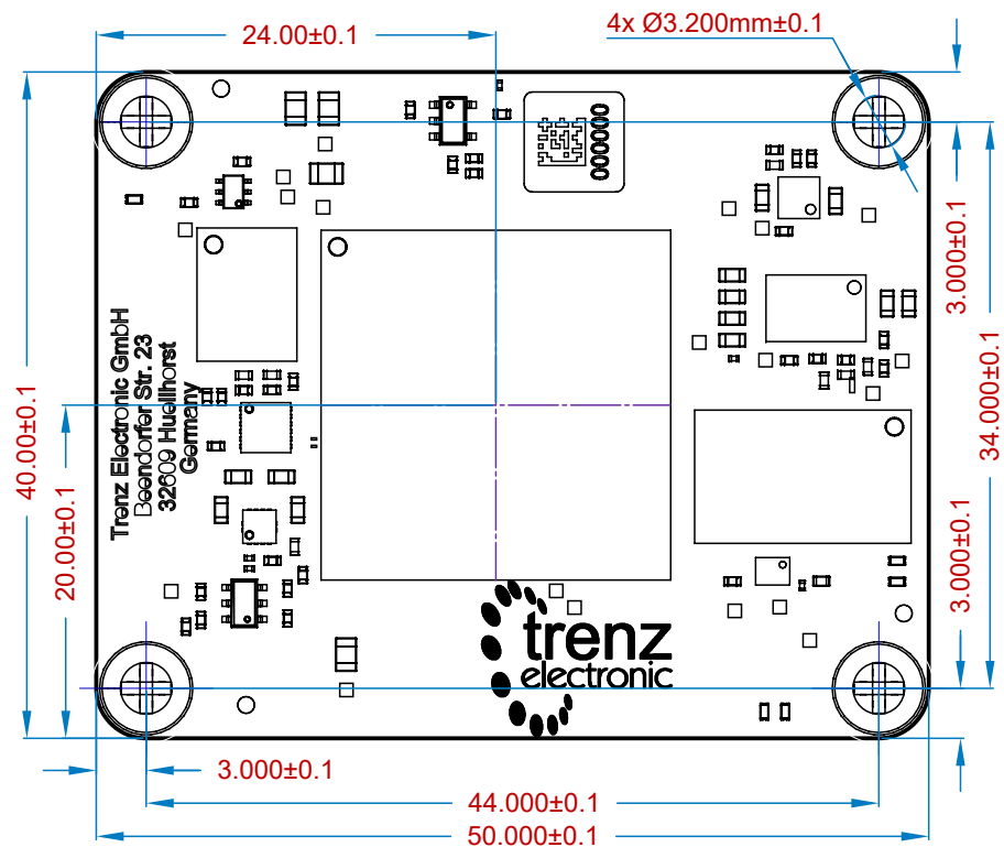
View from Top side (Scale 2:1)
