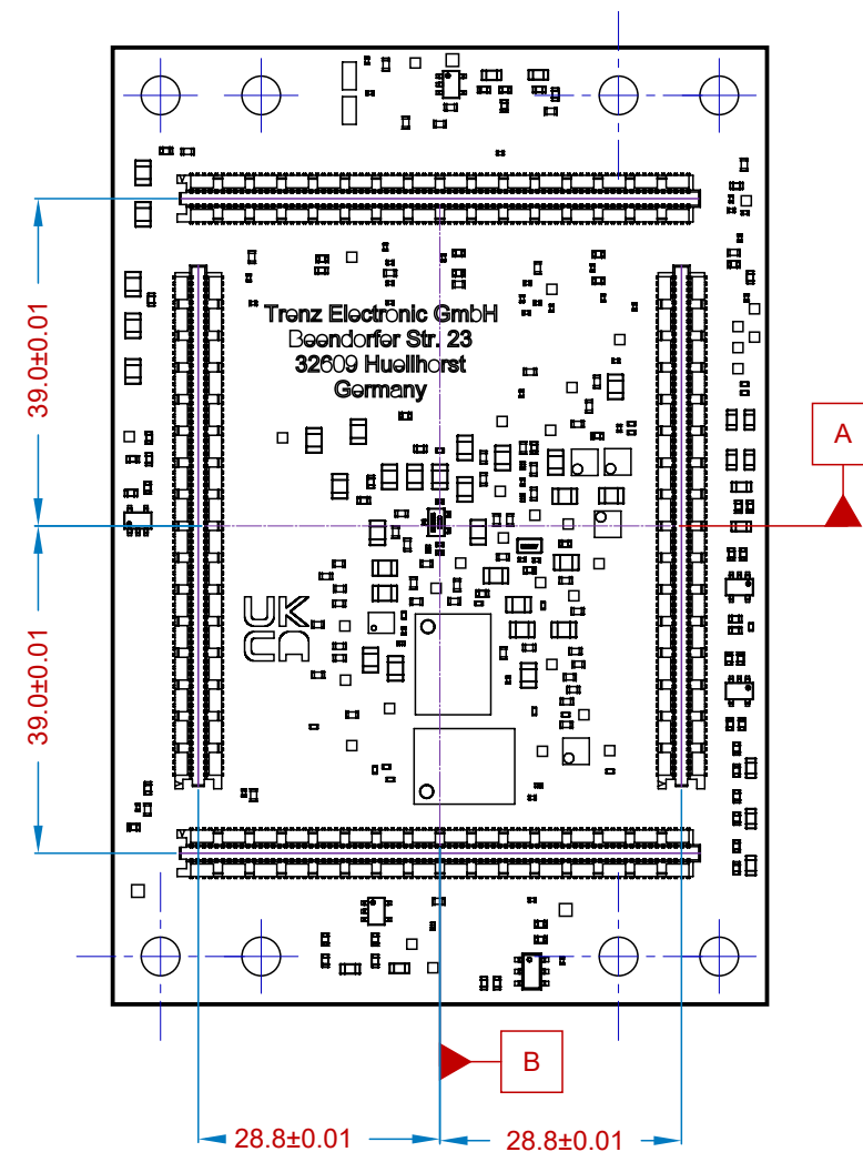
View from Bottom side (Scale 1.5:1)
