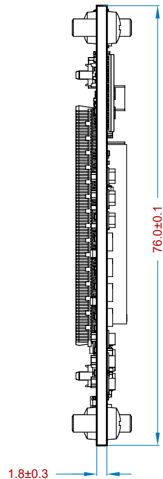
View from Left side (Scale 1.5:1)
