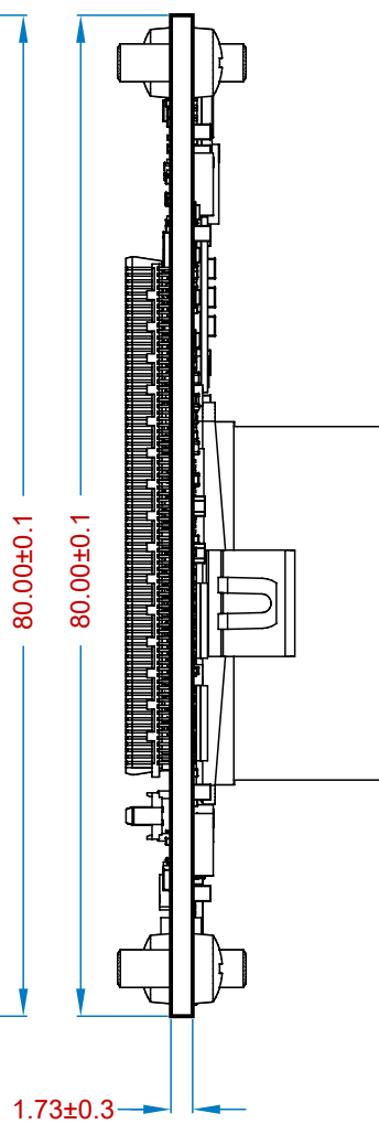
View from Left side (Scale 1.5:1)
