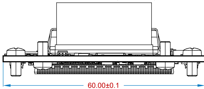
View from Front side (Scale 1.5:1)
