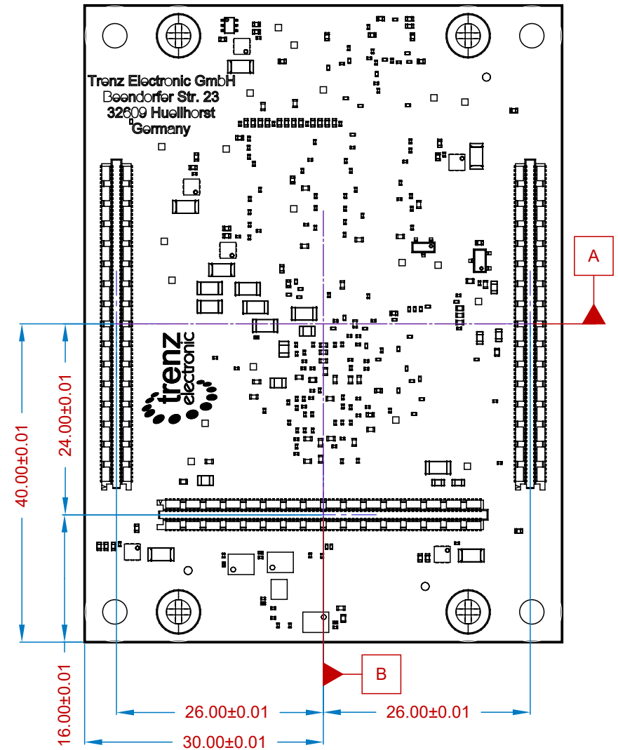
View from Bottom side (Scale 1.5:1)
