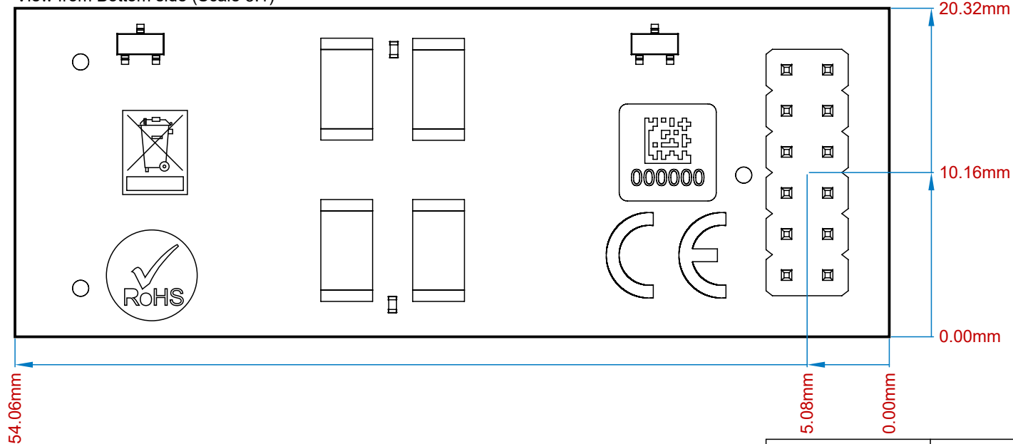
View from Bottom side (Scale 3:1)
