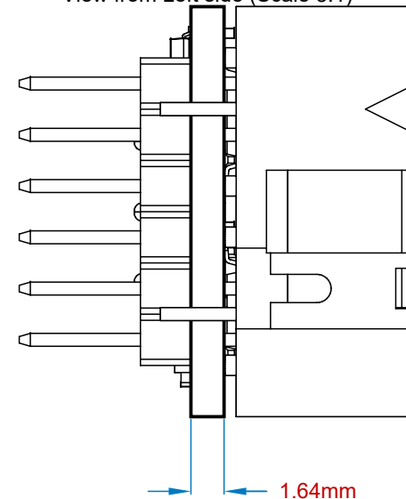
View from Left side (Scale 3:1)
